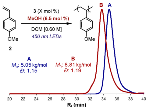
Figure 6. GPC trace showing monomodal molecular weight shift after monomer addition. Conditions: 2.5 mol % 3 , 6.5 mol % methanol, [0.60 M] 2 in DCM, blue LED irradiation. (A) Quenched with triethylamine after 10 min irradiation. (B) Irradiation ceased at 10 min, immediate addition of a further equivalent of 2 .
