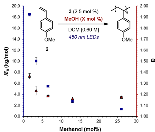
Figure 3. Influence of methanol loading on M_n (■) and \mathcal{D} (▲) of poly(4-methoxystyrene). M_n and \mathcal{D} were determined by GPC relative to polystyrene standards, average of three experiments. Conditions: 2.5 mol % 3 , [0.60 M] 2 in DCM, blue LED irradiation.
