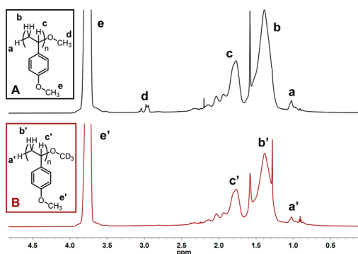
Figure 2. ^1\text{H} NMR spectra of poly(4-methoxystyrene). Conditions: 2.5 mol % 3 , 6.5 mol % methanol (A) or methanol- d 3 (B), [0.60 M] 2 in DCM, blue LED irradiation. (A) M_n = 5.35 kg/mol, \mathcal{D} = 1.18 or methanol- d 3 , (B) M_n = 6.26 kg/mol, \mathcal{D} = 1.15.
